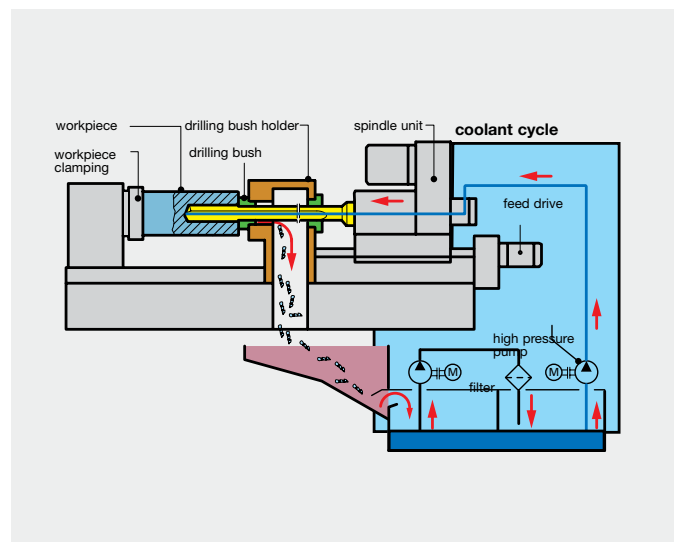
Gun drilling machines
